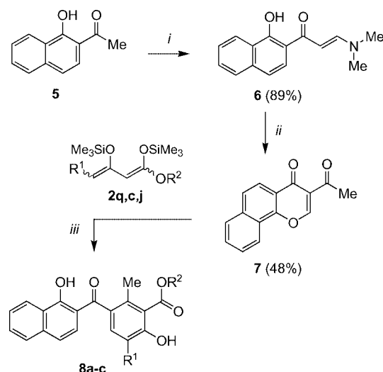
Scheme 4. Synthesis of 8a–c : i) 5 (1.0 equiv.), diethoxy- N,N -dimethylmethanamine (1.0 equiv.), 20 °C, 12 h; ii) Ac 2 O (4 equiv.), pyridine, MeCN, 6 h, reflux, then 12 h, 20 °C; iii) 1. Me 3 SiOTf (0.3 equiv.), 0 °C, 10 min, 2c,j,q (1.3 equiv.), CH 2 Cl 2 , 20 °C, 12 h; 2) HCl (10%).
