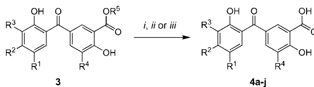
Scheme 3. Synthesis of 4a–j : i) 1. aqueous KOH (10%, 13.0 equiv.), DMSO, 20 °C, 12 h; 2. aqueous HCl (1 M); ii) 1. aqueous KOH (2 M, 4.0 equiv.), 20 °C, 36 h; 2. aqueous HCl (10%); iii) 1. BBr 3 (4.0 equiv.), CH 2 Cl 2 , 0 → 20 °C, 12 h; 2. aqueous HCl (10%).
