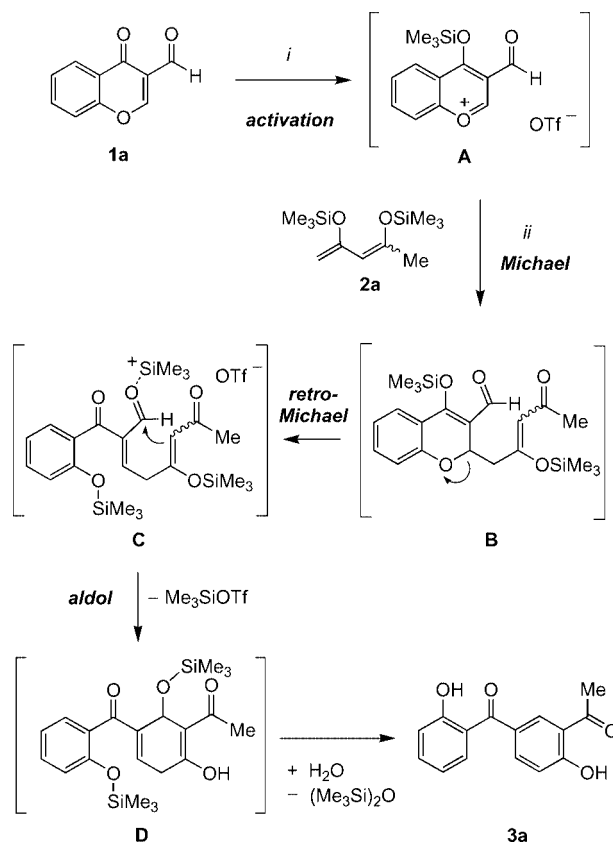
Scheme 1. Mechanism of the formation of 3a : i) \text{Me}_3\text{SiOTf} (0.3 equiv.), 20^\circ\text{C} , 10 min; ii) 1. 2a (1.3 equiv.), \text{CH}_2\text{Cl}_2 , 0 \rightarrow 20^\circ\text{C} , 12 h; 2. HCl (10%).
