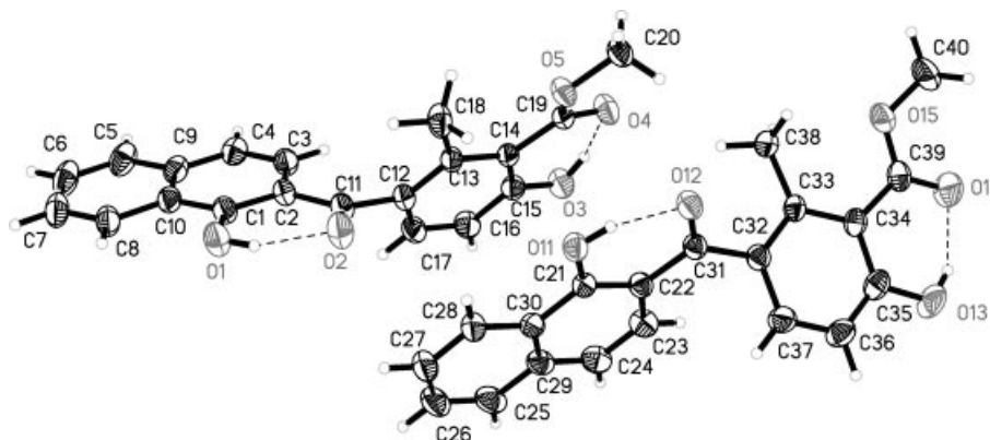
Figure 2. ORTEP plot of 8a . Selected bond lengths [Å] and angles [°]: C(1)–O(1) 1.3375(16), C(2)–C(11) 1.4668(16), C(11)–O(2) 1.2437(18), C(11)–C(12) 1.4975(18), C(12)–C(17) 1.3990(19), C(14)–C(15) 1.4153(16), C(14)–C(19) 1.4825(15), C(15)–O(3) 1.3518(16), C(19)–O(4) 1.2279(15), C(19)–O(5) 1.3238(14), C(39)–O(14) 1.2267(16), C(39)–O(15) 1.3179(18), C(40)–O(15) 1.4457(18), O(1)–H(1) 0.8400, O(3)–H(3A) 0.8400, O(11)–H(11) 0.8400, O(13)–H(13) 0.8400; O(1)–C(1)–C(2) 122.57(11), O(1)–C(1)–C(10) 116.56(11), C(2)–C(1)–C(10) 120.87(12).
