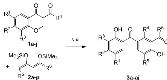
Scheme 2. Synthesis of 3a–aj : i) \text{Me}_3\text{SiOTf} (0.3 equiv.) 20^\circ\text{C} , 10 min; ii) 1. 2a–p (1.3 equiv.), \text{CH}_2\text{Cl}_2 , 0 \rightarrow 20^\circ\text{C} , 12 h; 2. HCl (10%).
