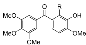
Phenstatin (R = H) Antitubulin agents (R = OH, NH 2 )
