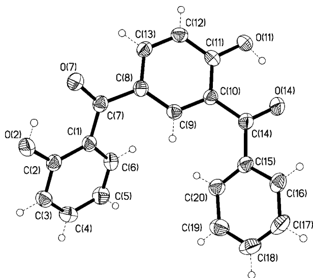
Figure 1. ORTEP plot of 3b .
